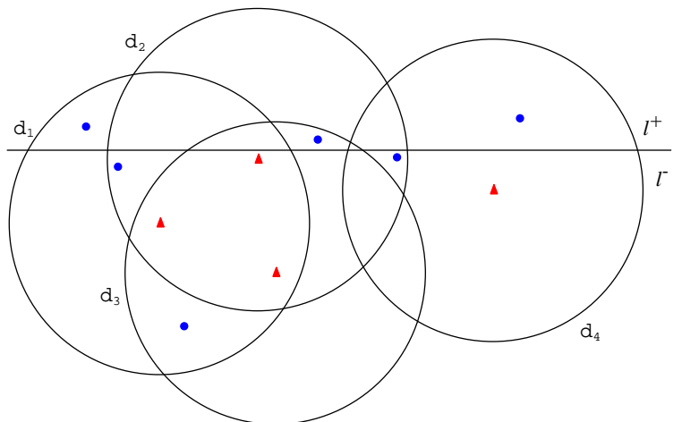
Fig. 1. Demonstration of the arrangement of circles centered at points indicated by triangles.
