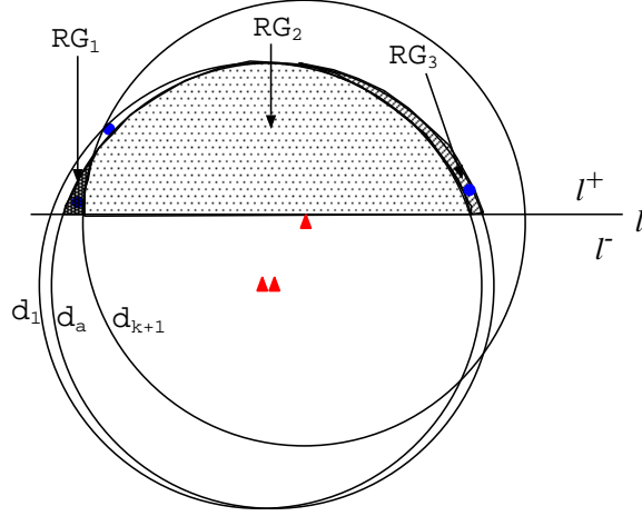
Fig. 2. Illustration in support of Theorem 2.2.
