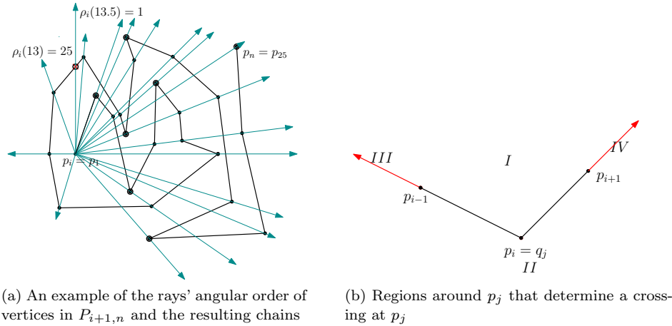
Fig. 3: Angular ordering with chains around p_i and regions local to p_i
