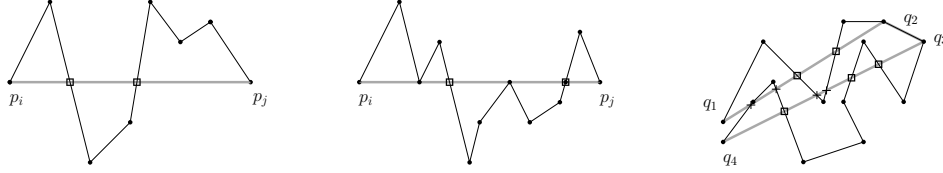
Fig. 1: Crossings are indicated with a square and false crossings are marked with a +. Crossings are only counted when the simplifying segment intersects the chain that begins and ends with its own endpoints.
