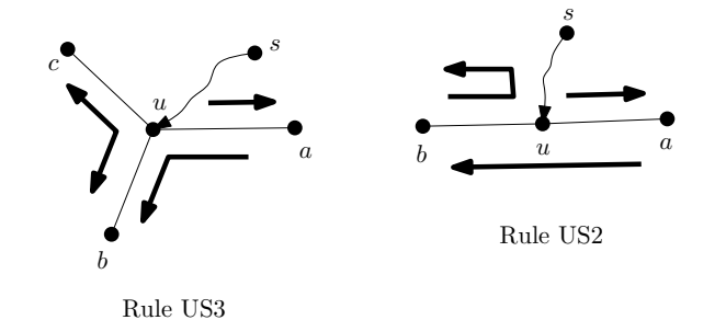
Figure 9: Algorithm 1, Case 4: Message received/forwarded by a node u that cannot see t and sees s in a passive component.
