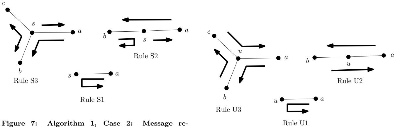
Figure 7: Algorithm 1, Case 2: Message received/forwarded by s .
