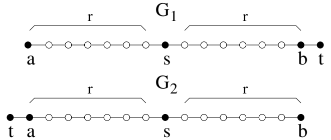
Figure 5: illustration in support of Theorem 5
