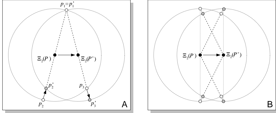
Figure 4.2: illustrations supporting Thm. 4.2 (reproduced from [BBKS00])
