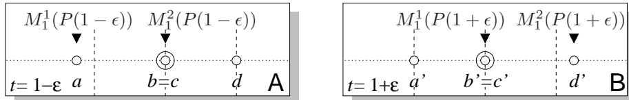
Figure 7.2: illustration in support of Thm. 7.2
