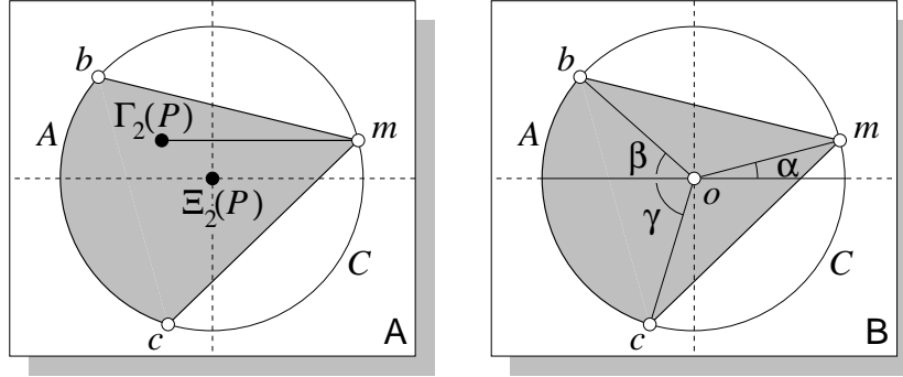
Figure 4.20: Thm. 4.20: maximizing the eccentricity of the Steiner centre
