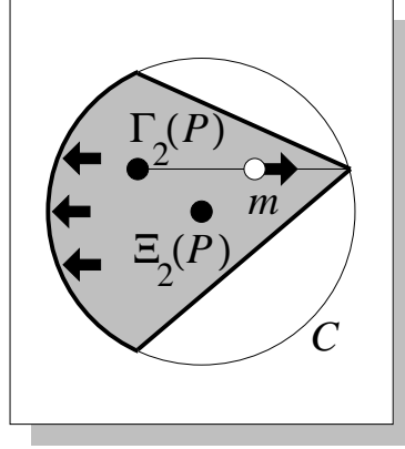
Figure 4.19: illustrations supporting Lem. 4.19
