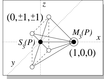
Figure 5.4: example realizing the lower bound of the approximation factor on the rectilinear 1-median in \mathbb{R}^3
