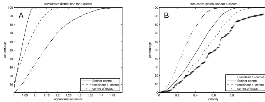
Figure 8.9: centre function cumulative plots for approximation factor and average velocity for six mobile clients
