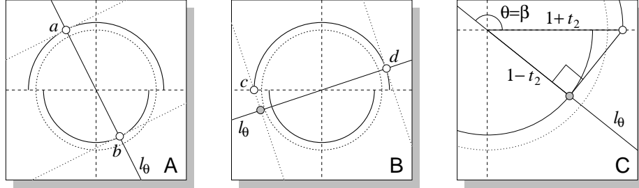
Figure 4.22: illustrations supporting Thm. 4.25
