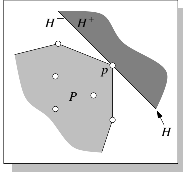
Figure 4.5: Point p is an extreme point of set P .
