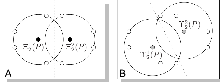
Figure 6.5: different partitions induced by \Xi_2 and \Upsilon_2
