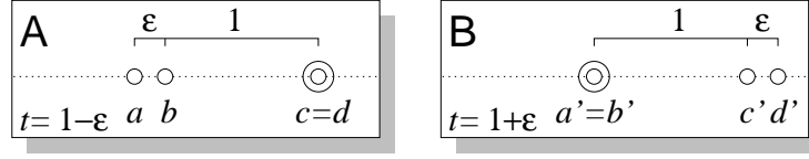
Figure 7.1: illustration in support of Thm. 7.1
