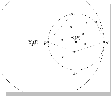
Figure 4.3: Centre function \Upsilon_2(P) = p has eccentricity 2 and maximum velocity 1, where p is a client in P .
