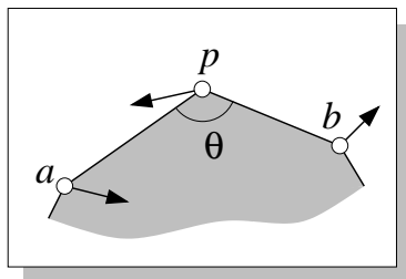
Figure 8.1: The Gaussian weight of client p is defined in terms of the positions of clients p , a , and b .
