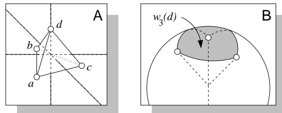
Figure 4.15: the Gauss map in three dimensions
