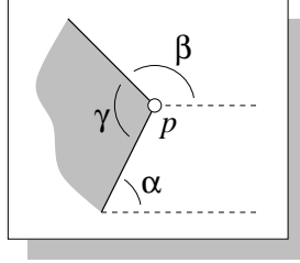
Figure 4.11: alternative definition for the Gaussian weight of p
