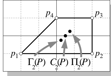
Figure 5.13: As a consequence of Cor. 5.30 and Thm. 5.31, C_2(P) = \frac{1}{2}[\Gamma_2(P) + \Pi_2(P)] when |P| = 4 .
