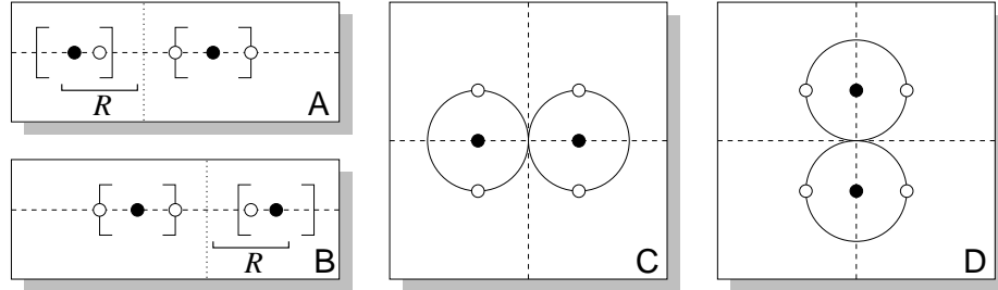
Figure 6.1: non-uniqueness of the geometric 2-centre in \mathbb{R} and the Euclidean 2-centre in \mathbb{R}^2
