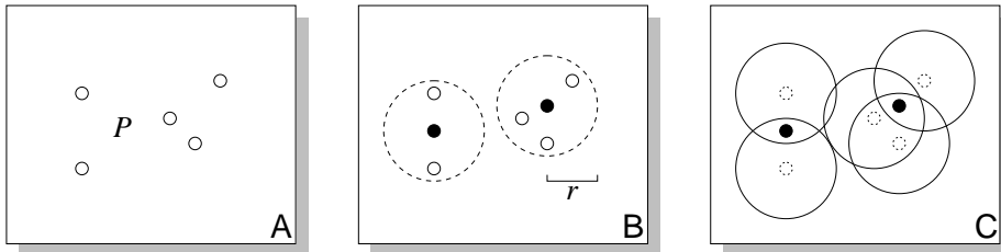
Figure 2.11: A. a set of points P in \mathbb{R}^2 , B. a Euclidean 2-centre of P of radius r , C. the corresponding 2-piercing for a set of disc of radius r centred at the points of P
