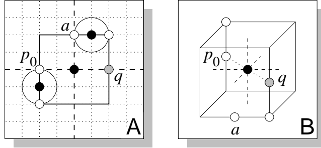
Figure 6.11: illustration in support of Thm. 6.24
