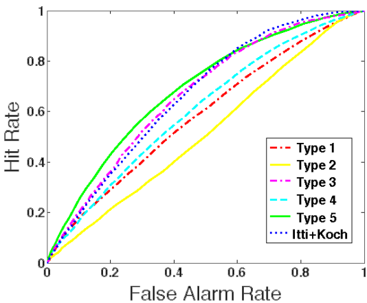
Fig. 4. ROC curves for the various operators.
